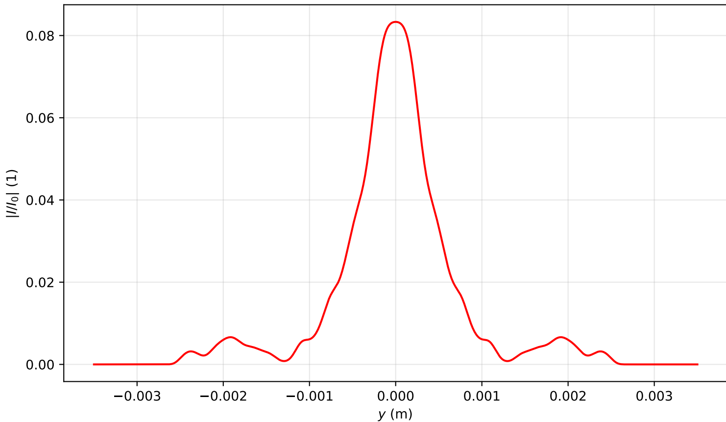
Intensity profile I(x = 0, y, z = 2.388)/I_0 , P_{in}=11.0\text{Pcr} , artificial time
