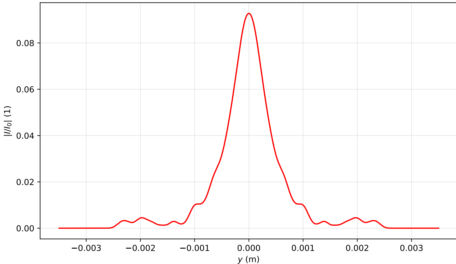
Intensity profile I(x=0, y, z=2.548)/I_0 , P_{in}=11.0P_{cr} , artificial time
