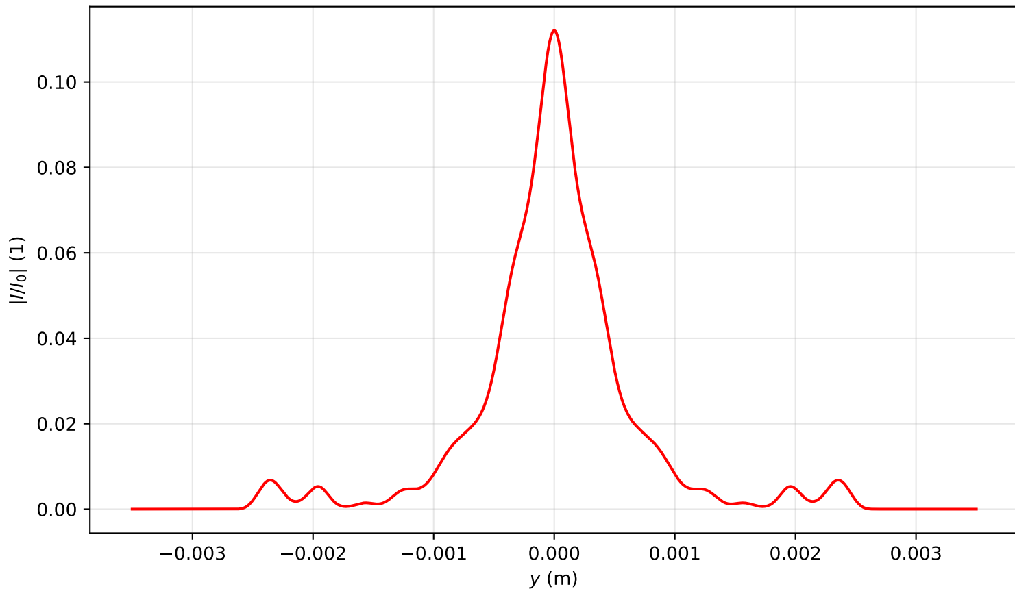
Intensity profile I(x = 0, y, z = 2.707)/I_0 , P_{in}=11.0P_{cr} , artificial time
