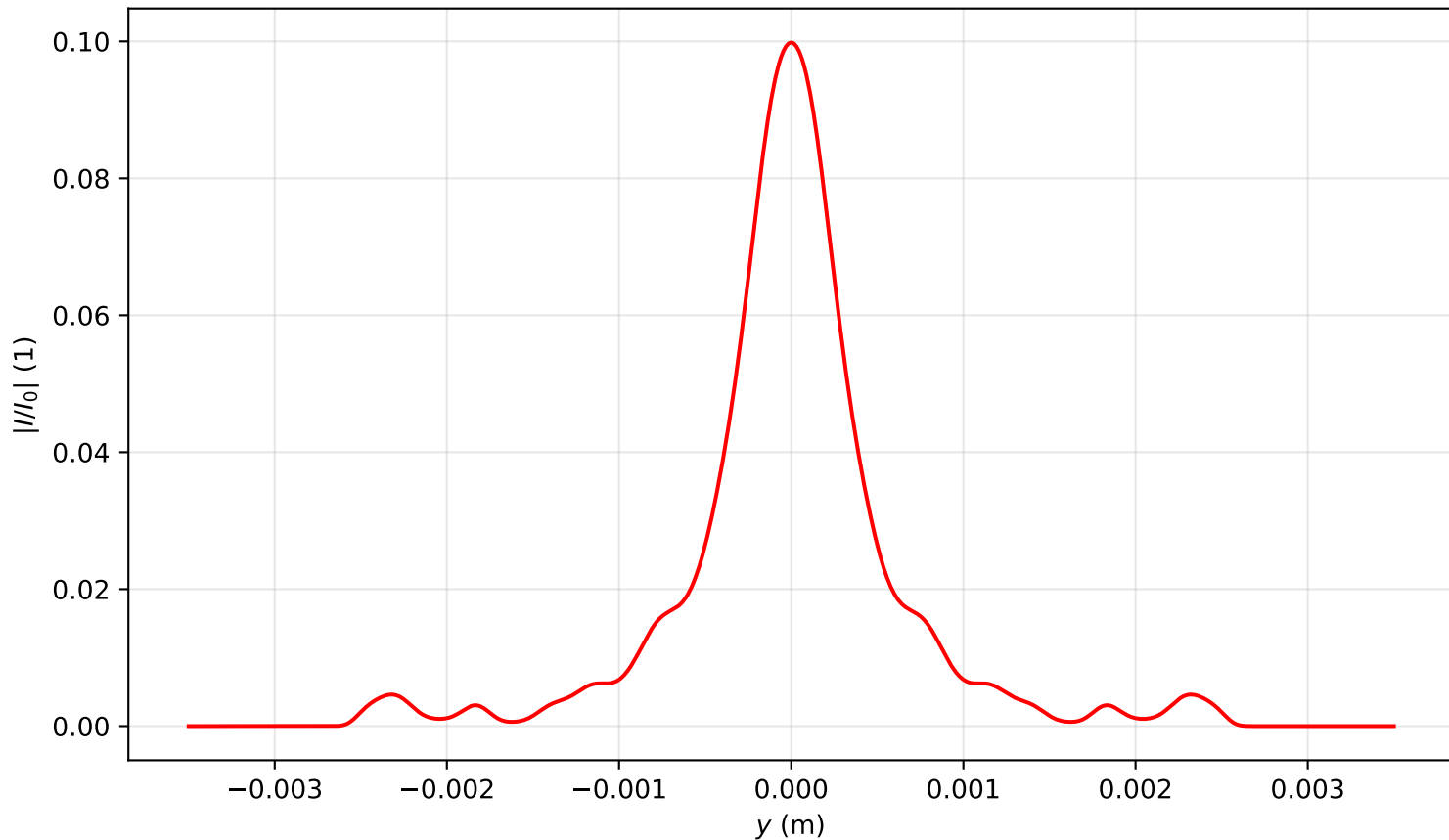
Intensity profile I(x = 0, y, z = 2.866)/I_0 , P_{in}=11.0P_{cr} , artificial time
