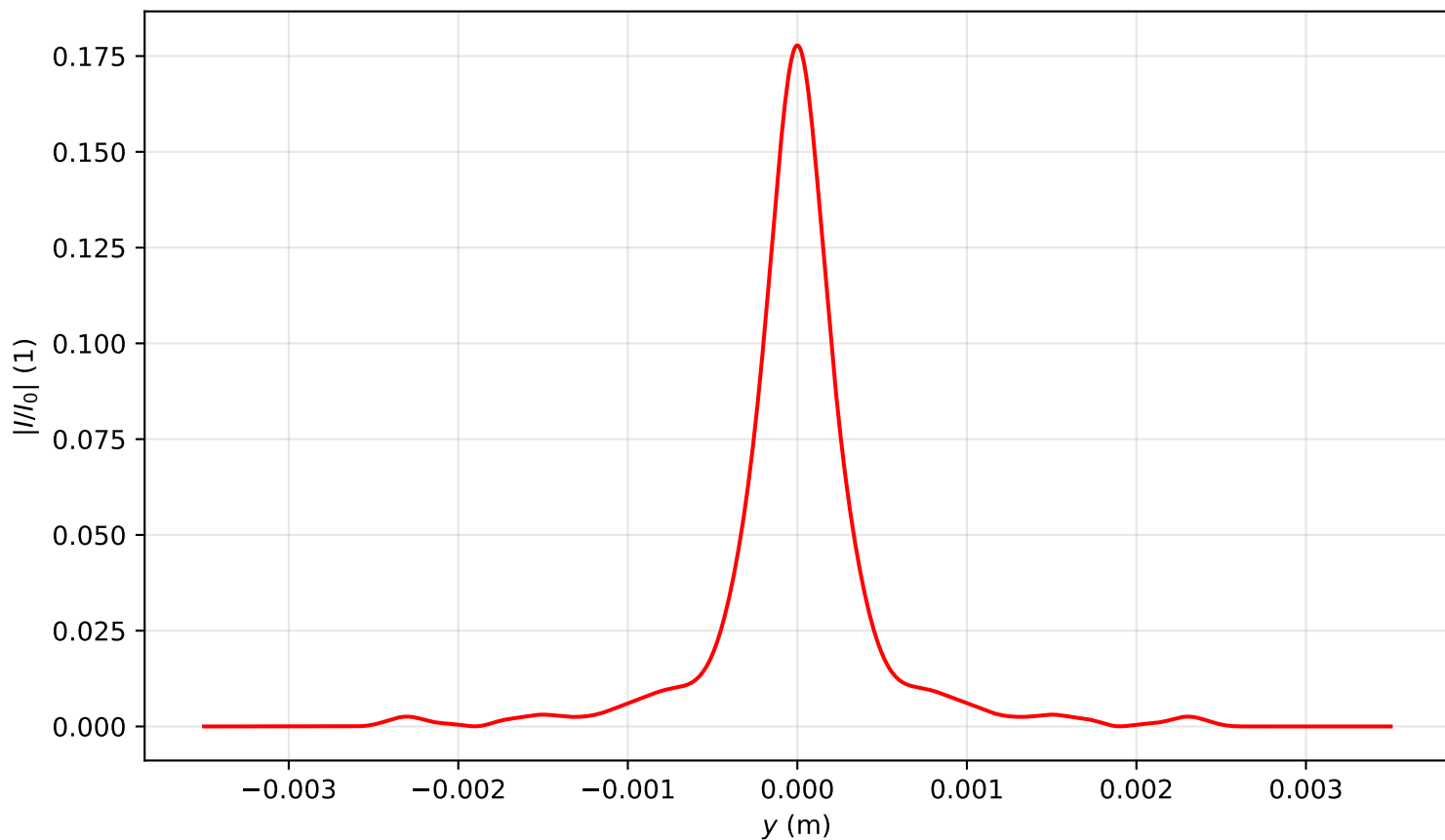
Intensity profile I(x=0, y, z=3.662)/I_0 , \text{Pin}=11.0\text{Pcr} , artificial time
