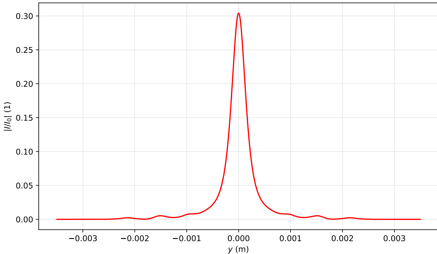
Intensity profile I(x=0, y, z=3.981)/I_0 , P_{in}=11.0P_{cr} , artificial time
