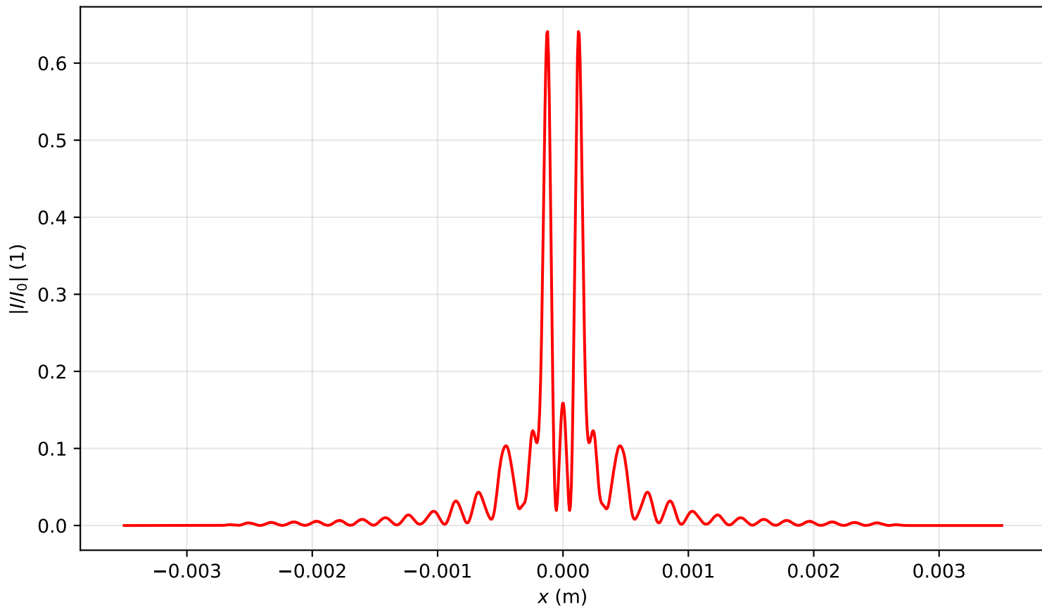
Intensity profile I(x, y = 0, z = 0.159)/I_0 , P_{in}=12.0P_{cr} , artificial time
