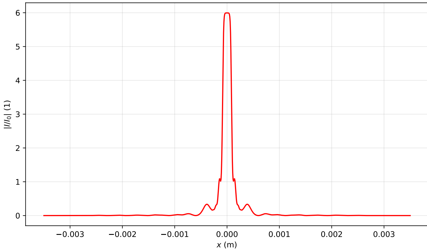
Intensity profile I(x, y = 0, z = 0.318)/I_0 , P_{in}=12.0P_{cr} , artificial time
