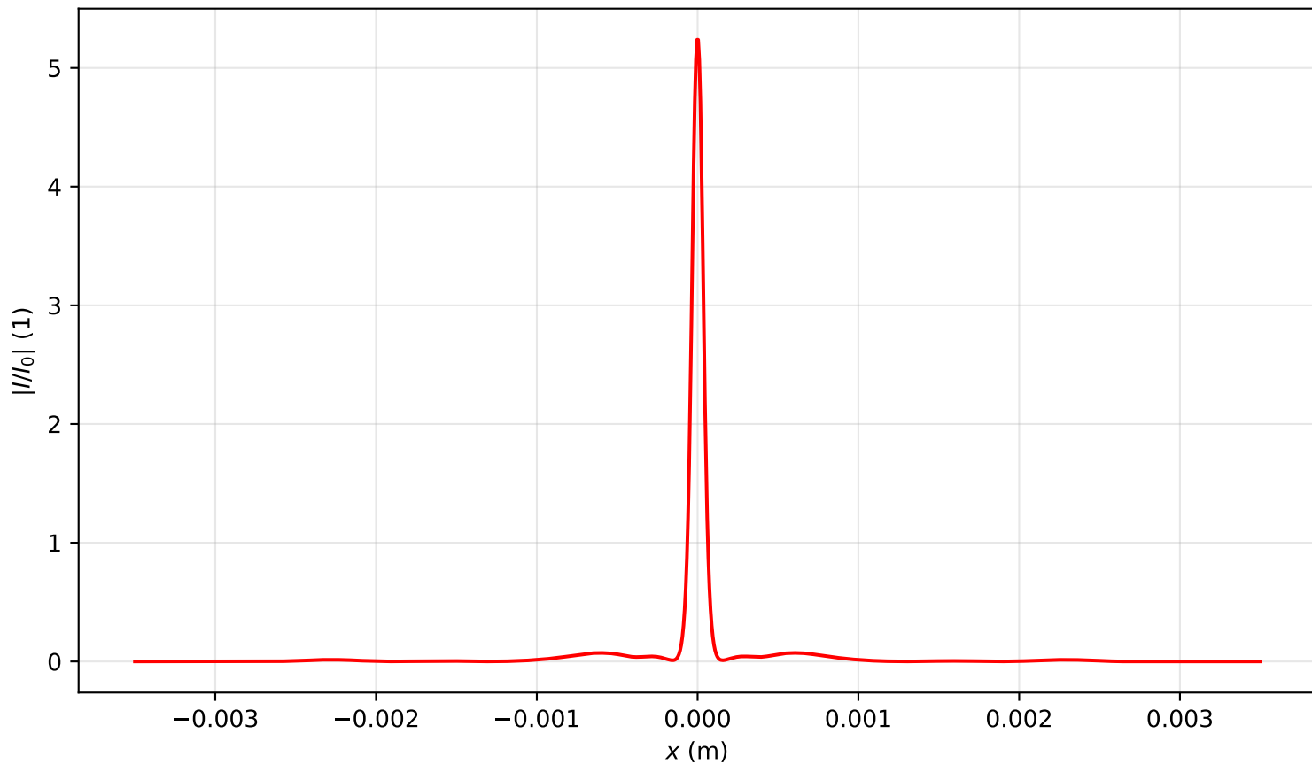
Intensity profile I(x, y = 0, z = 0.955)/I_0 , P_{in}=12.0P_{cr} , artificial time
