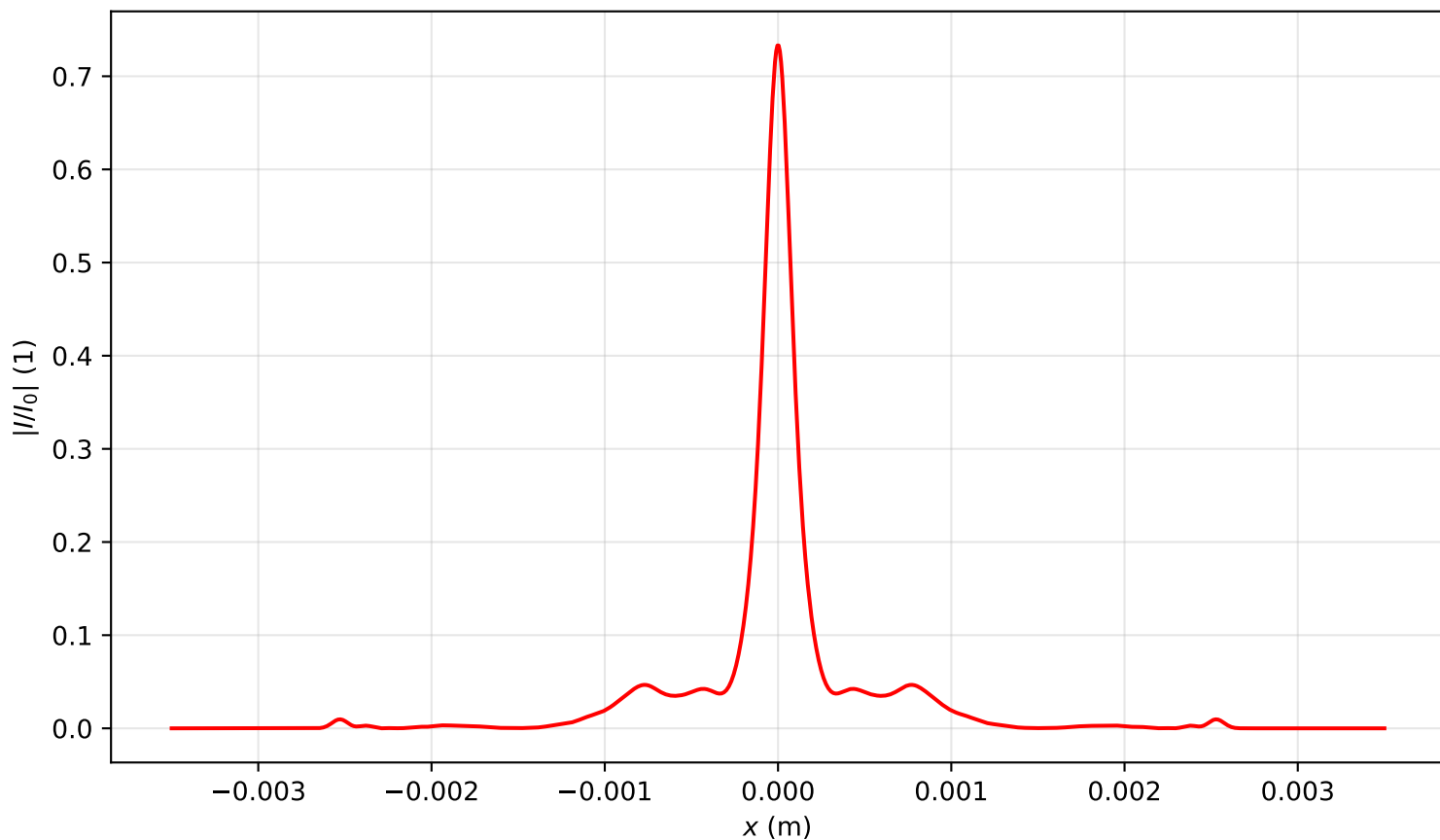
Intensity profile I(x, y = 0, z = 1.115)/I_0 , P_{in}=12.0P_{cr} , artificial time
