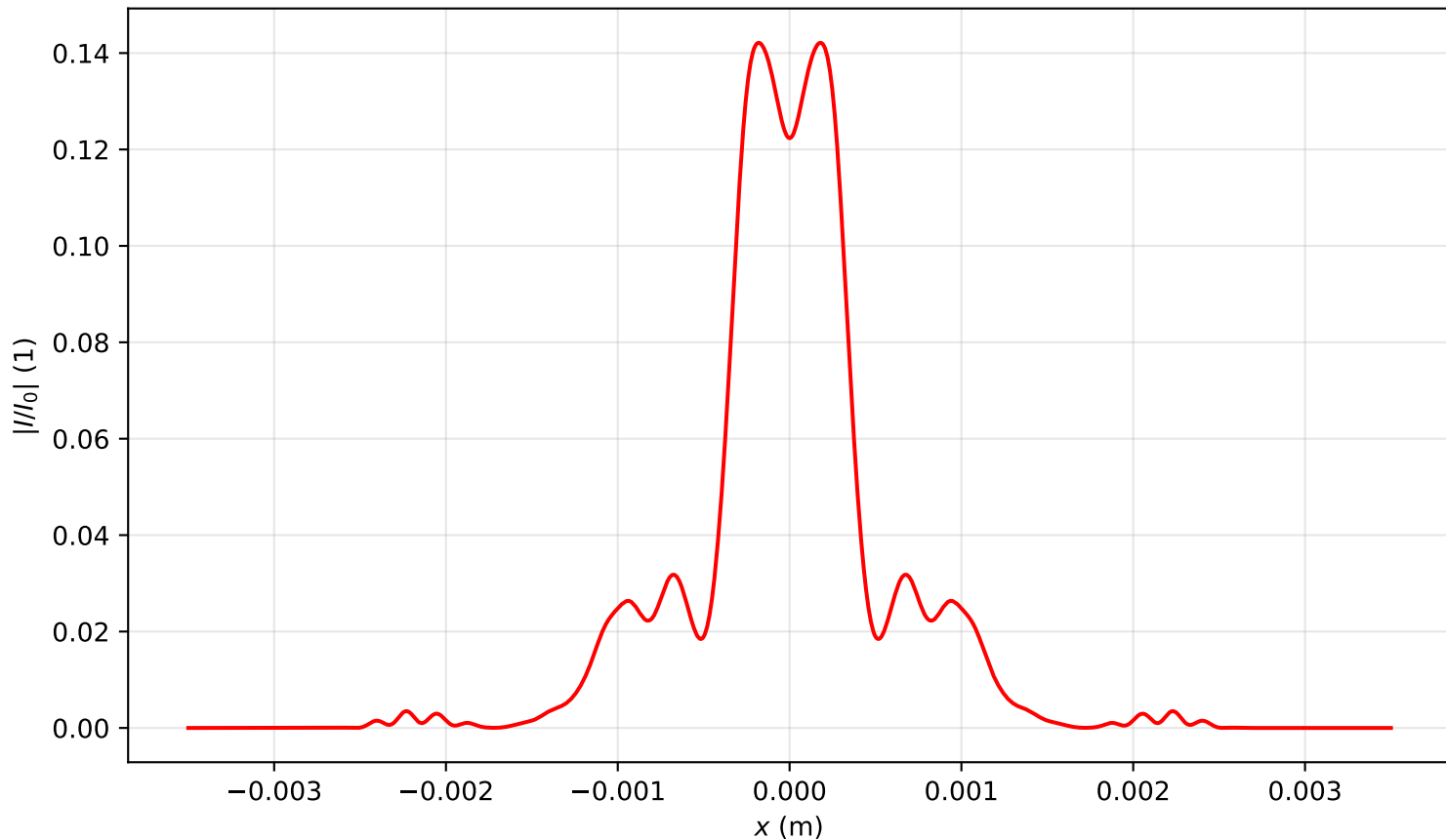
Intensity profile I(x, y = 0, z = 1.274)/I_0 , P_{in}=12.0\text{Pcr} , artificial time
