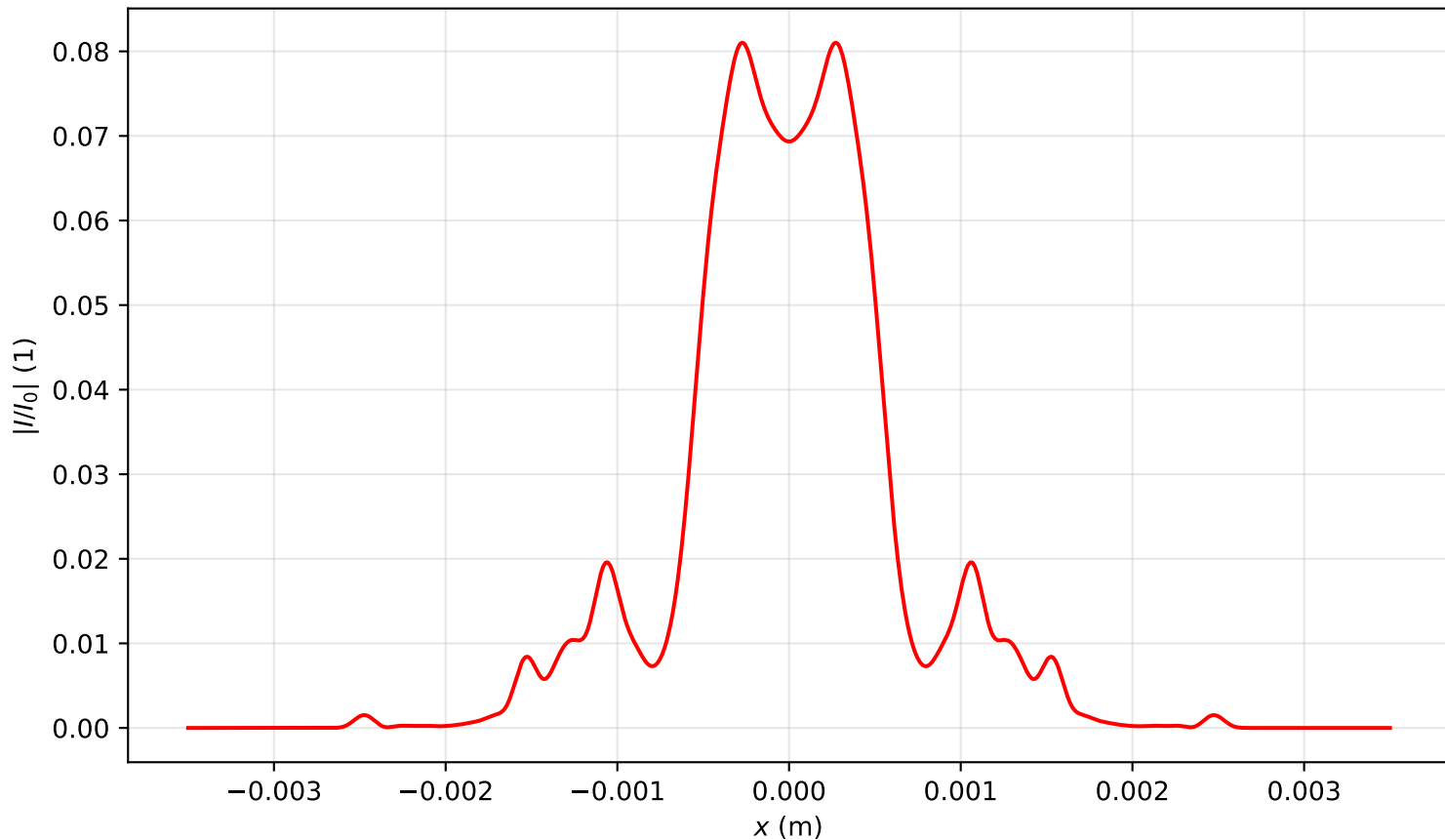
Intensity profile I(x, y = 0, z = 1.592)/I_0 , P_{in}=12.0P_{cr} , artificial time
