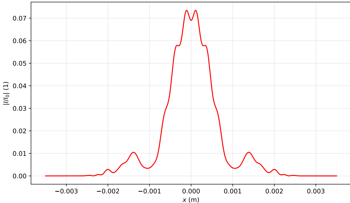
Intensity profile I(x, y = 0, z = 1.911)/I_0 , P_{in}=12.0P_{cr} , artificial time
