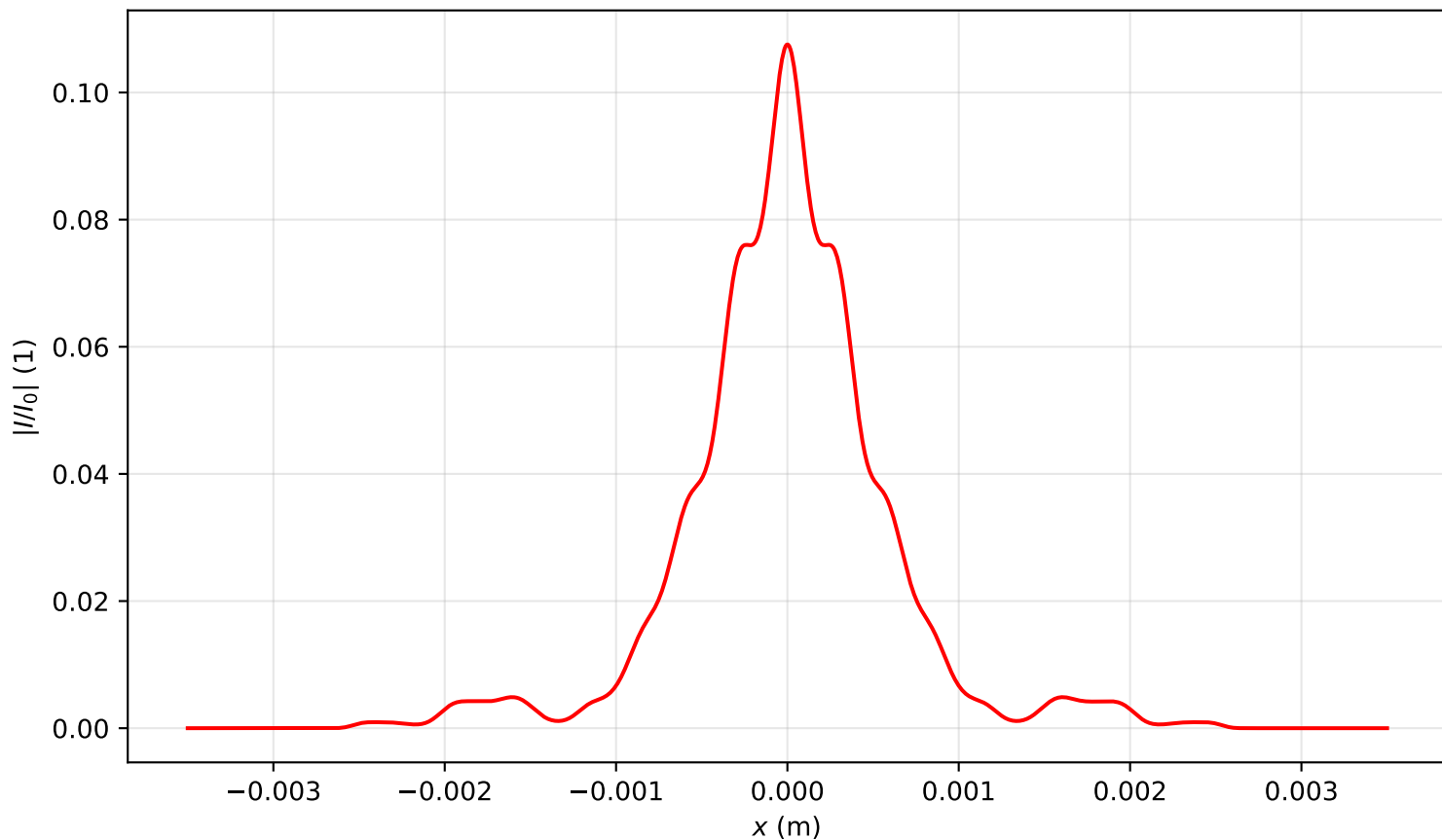
Intensity profile I(x, y = 0, z = 2.229)/I_0 , P_{in}=12.0P_{cr} , artificial time
