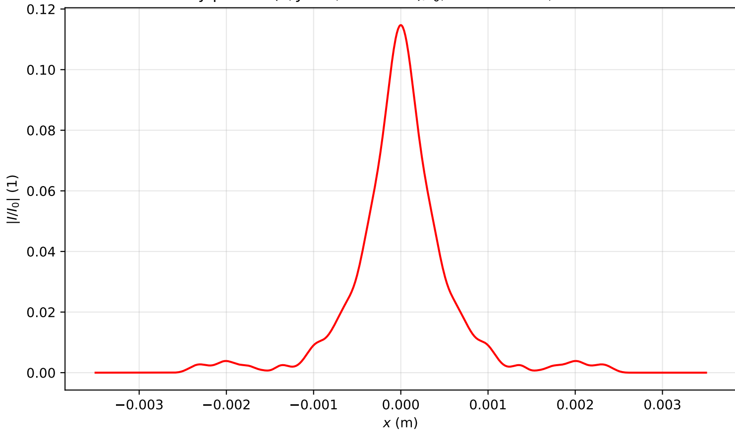
Intensity profile I(x, y = 0, z = 2.548)/I_0 , P_{in}=12.0\text{Pcr} , artificial time
