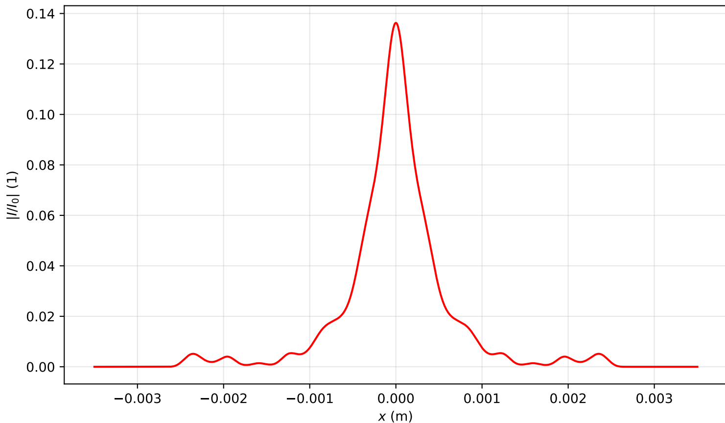
Intensity profile I(x, y = 0, z = 2.707)/I_0 , P_{in}=12.0P_{cr} , artificial time
