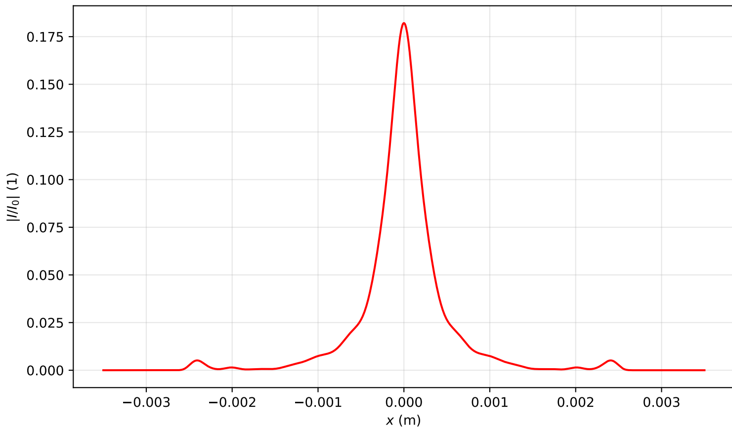
Intensity profile I(x, y = 0, z = 3.025)/I_0 , P_{in}=12.0P_{cr} , artificial time
