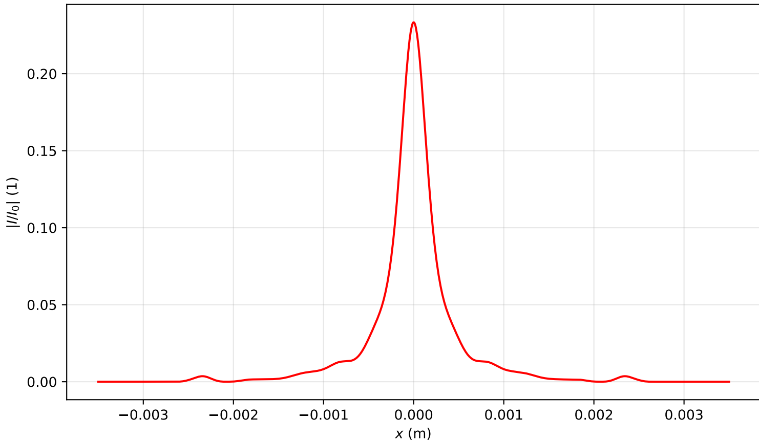
Intensity profile I(x, y = 0, z = 3.184)/I_0 , P_{in}=12.0P_{cr} , artificial time
