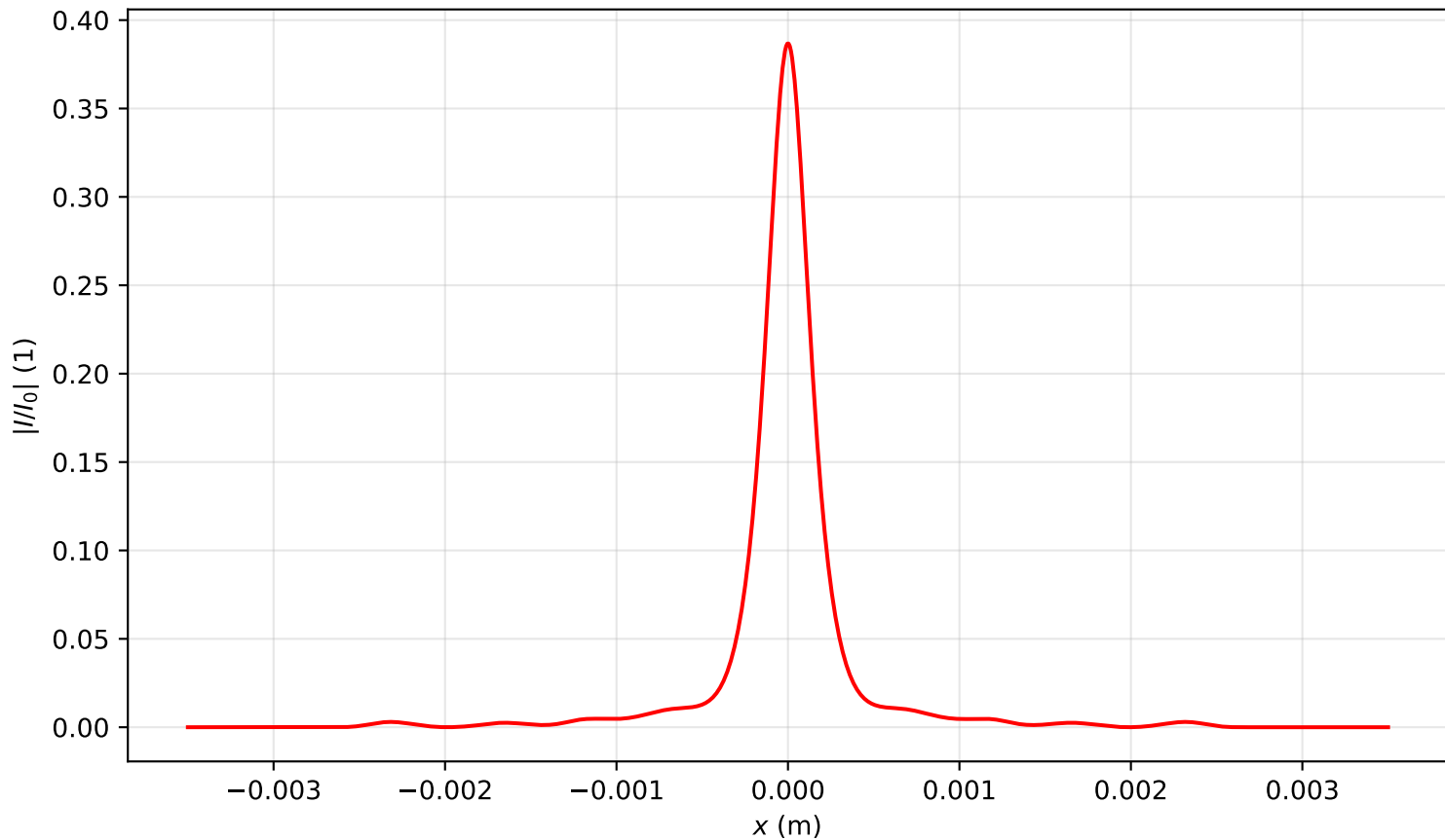
Intensity profile I(x, y = 0, z = 3.503)/I_0 , P_{in}=12.0P_{cr} , artificial time
