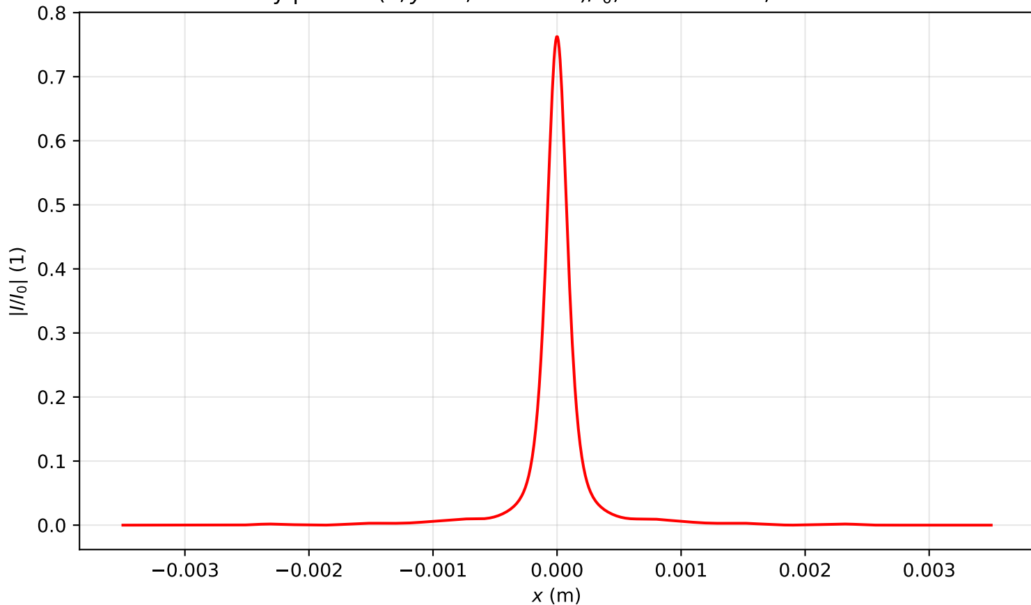
Intensity profile I(x, y = 0, z = 3.662)/I_0 , P_{in}=12.0P_{cr} , artificial time
