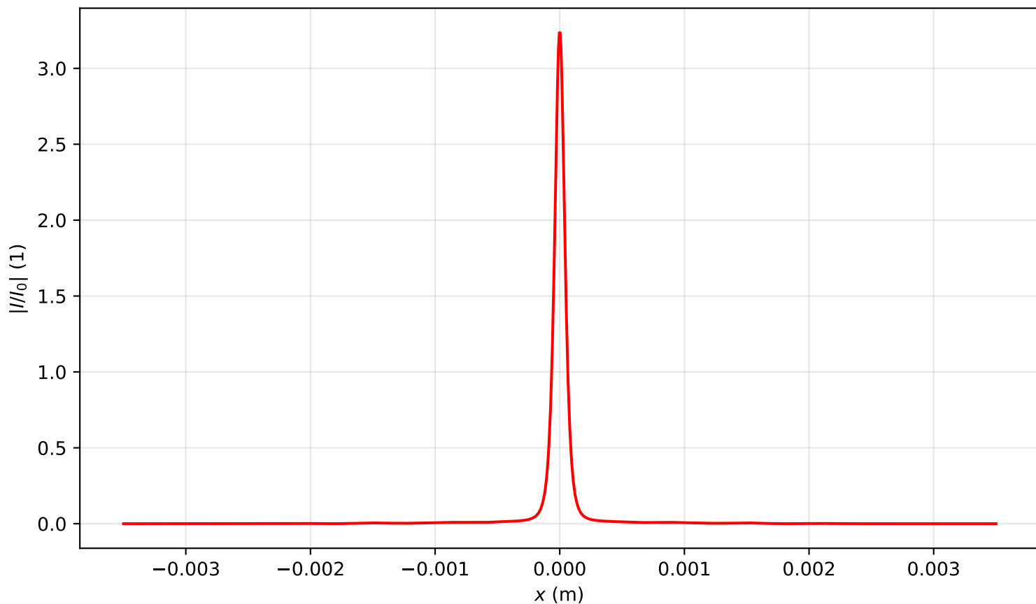
Intensity profile I(x, y = 0, z = 3.821)/I_0 , P_{in}=12.0P_{cr} , artificial time
