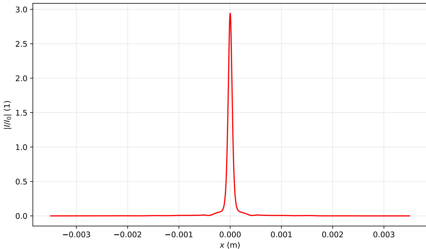
Intensity profile I(x, y = 0, z = 3.981)/I_0 , P_{in}=12.0P_{cr} , artificial time
