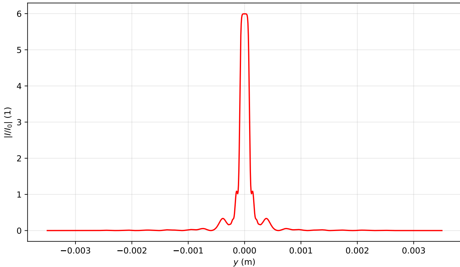
Intensity profile I(x=0, y, z=0.318)/I_0 , P_{in}=12.0P_{cr} , artificial time
