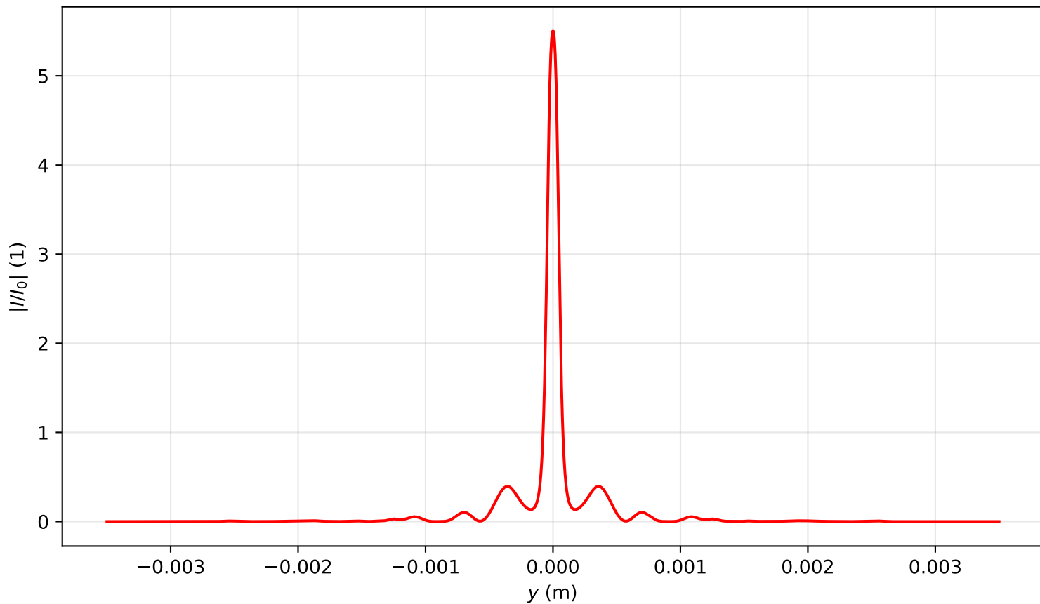
Intensity profile I(x=0, y, z=0.478)/I_0 , P_{in}=12.0P_{cr} , artificial time
