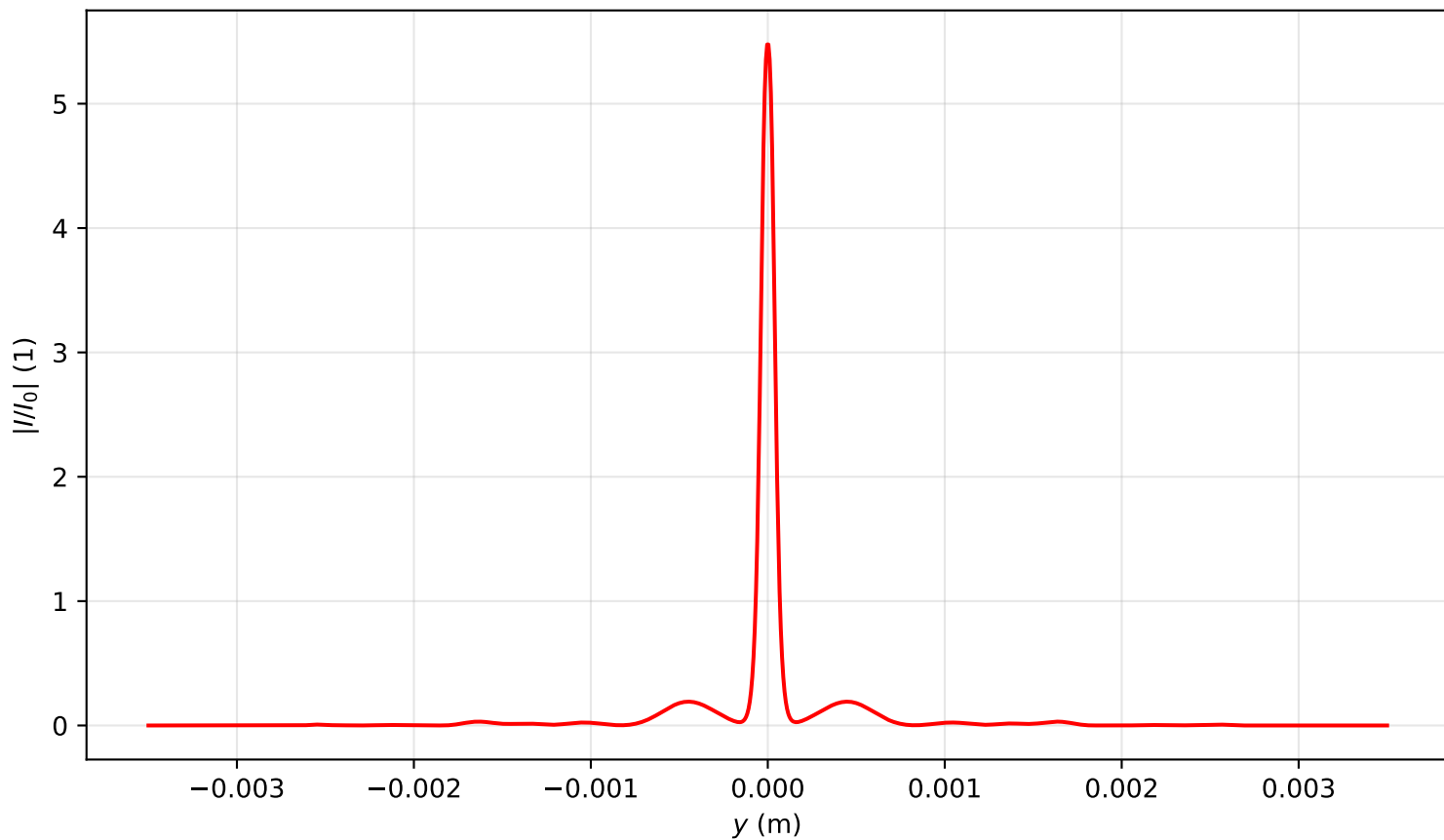
Intensity profile I(x=0, y, z=0.637)/I_0 , P_{in}=12.0P_{cr} , artificial time
