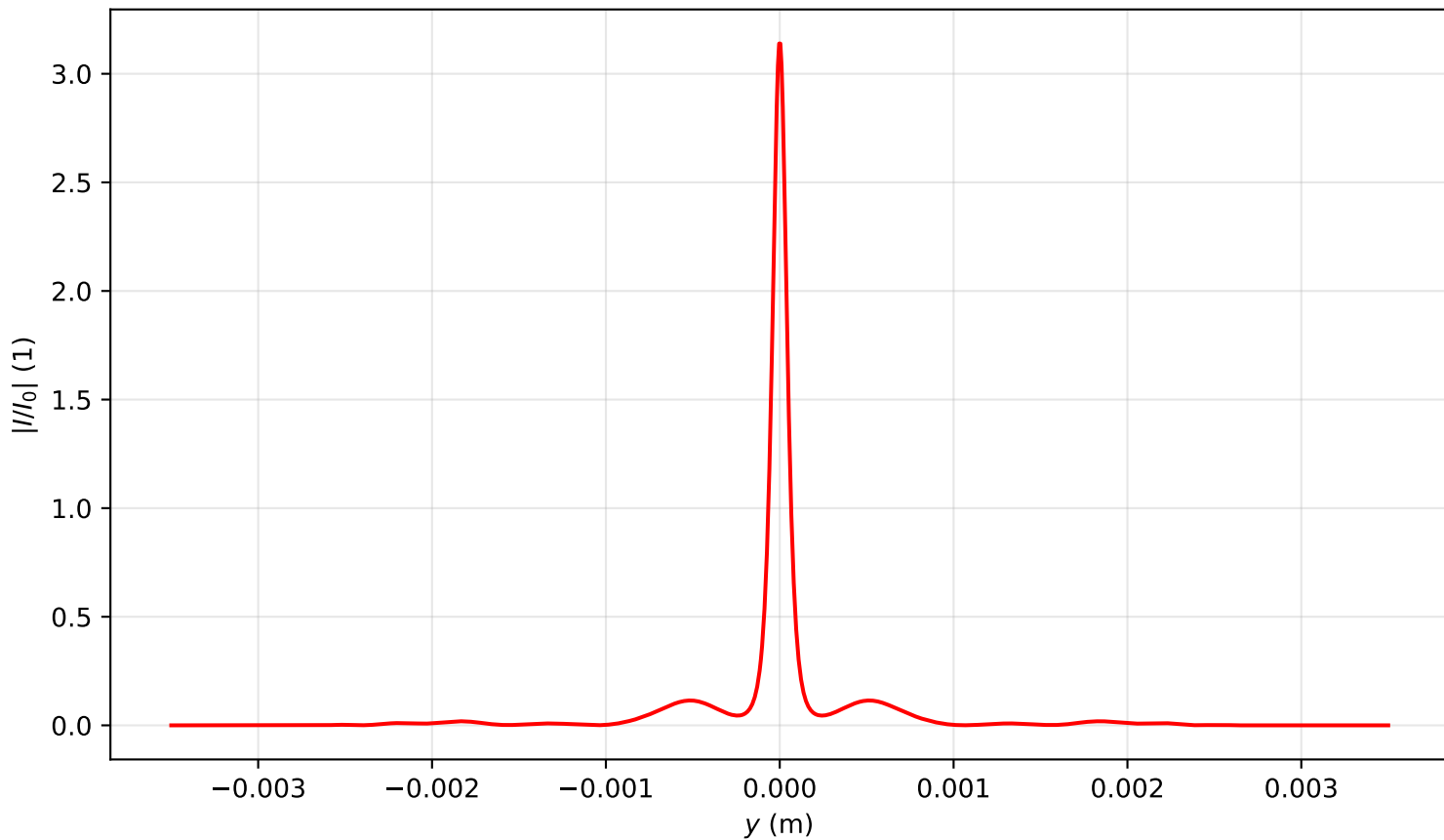
Intensity profile I(x=0, y, z=0.796)/I_0 , P_{in}=12.0P_{cr} , artificial time
