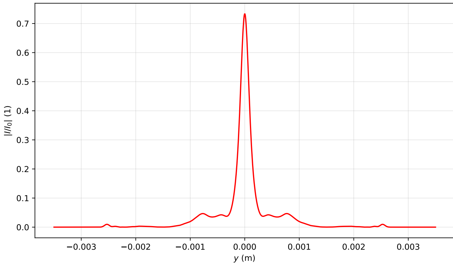
Intensity profile I(x=0, y, z=1.115)/I_0 , P_{in}=12.0P_{cr} , artificial time
