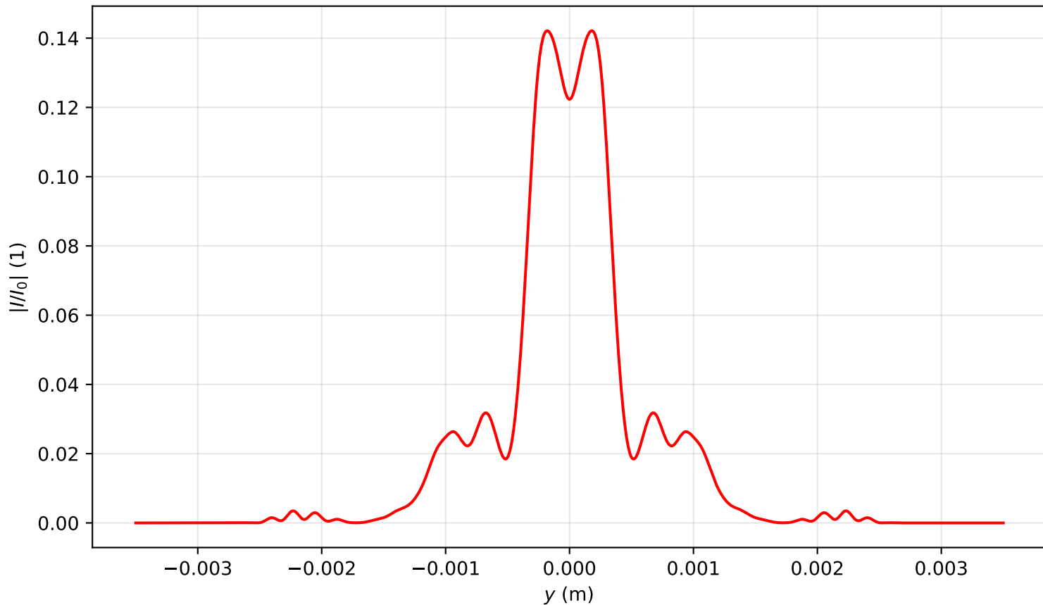
Intensity profile I(x=0, y, z=1.274)/I_0 , P_{in}=12.0\text{Pcr} , artificial time
