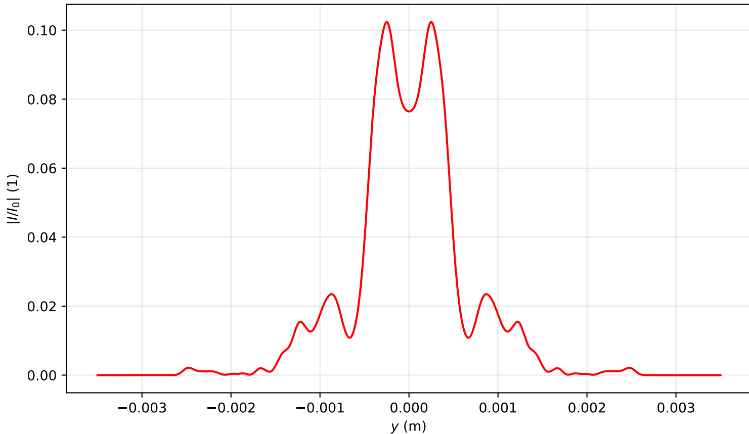
Intensity profile I(x = 0, y, z = 1.433)/I_0 , P_{in}=12.0P_{cr} , artificial time
