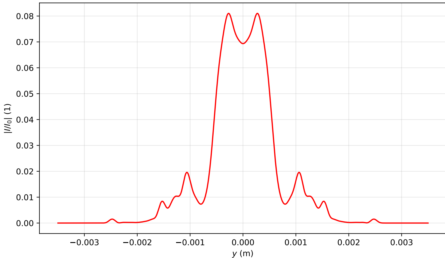
Intensity profile I(x = 0, y, z = 1.592)/I_0 , P_{in}=12.0P_{cr} , artificial time
