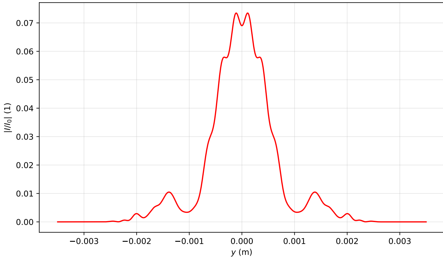
Intensity profile I(x=0, y, z=1.911)/I_0 , P_{in}=12.0\text{Pcr} , artificial time
