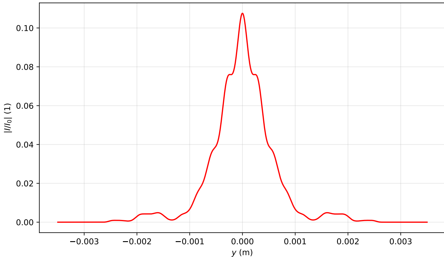
Intensity profile I(x = 0, y, z = 2.229)/I_0 , P_{in}=12.0P_{cr} , artificial time
