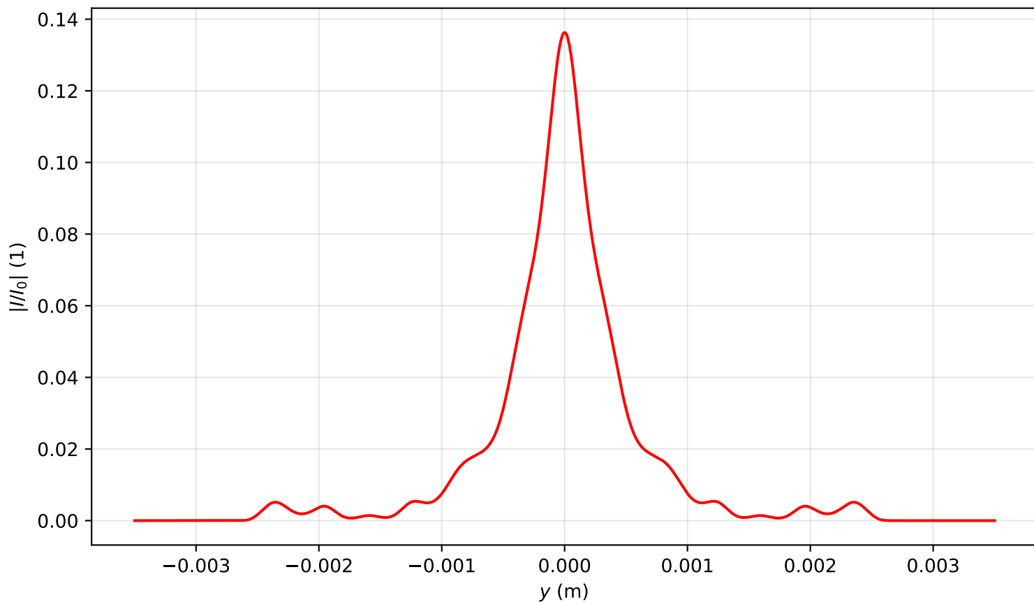
Intensity profile I(x=0, y, z=2.707)/I_0 , P_{in}=12.0P_{cr} , artificial time
