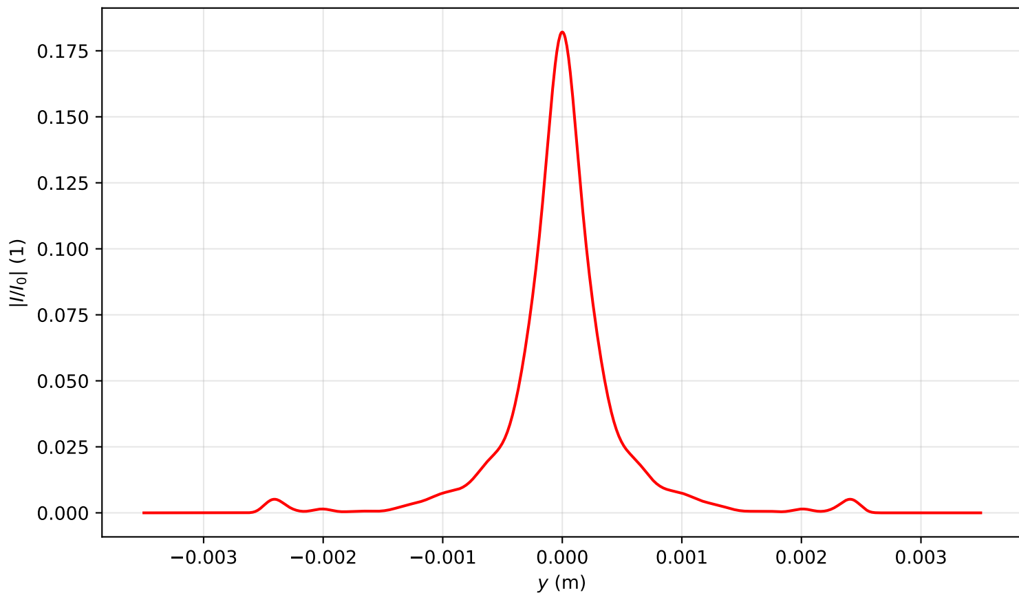
Intensity profile I(x=0, y, z=3.025)/I_0 , P_{in}=12.0P_{cr} , artificial time
