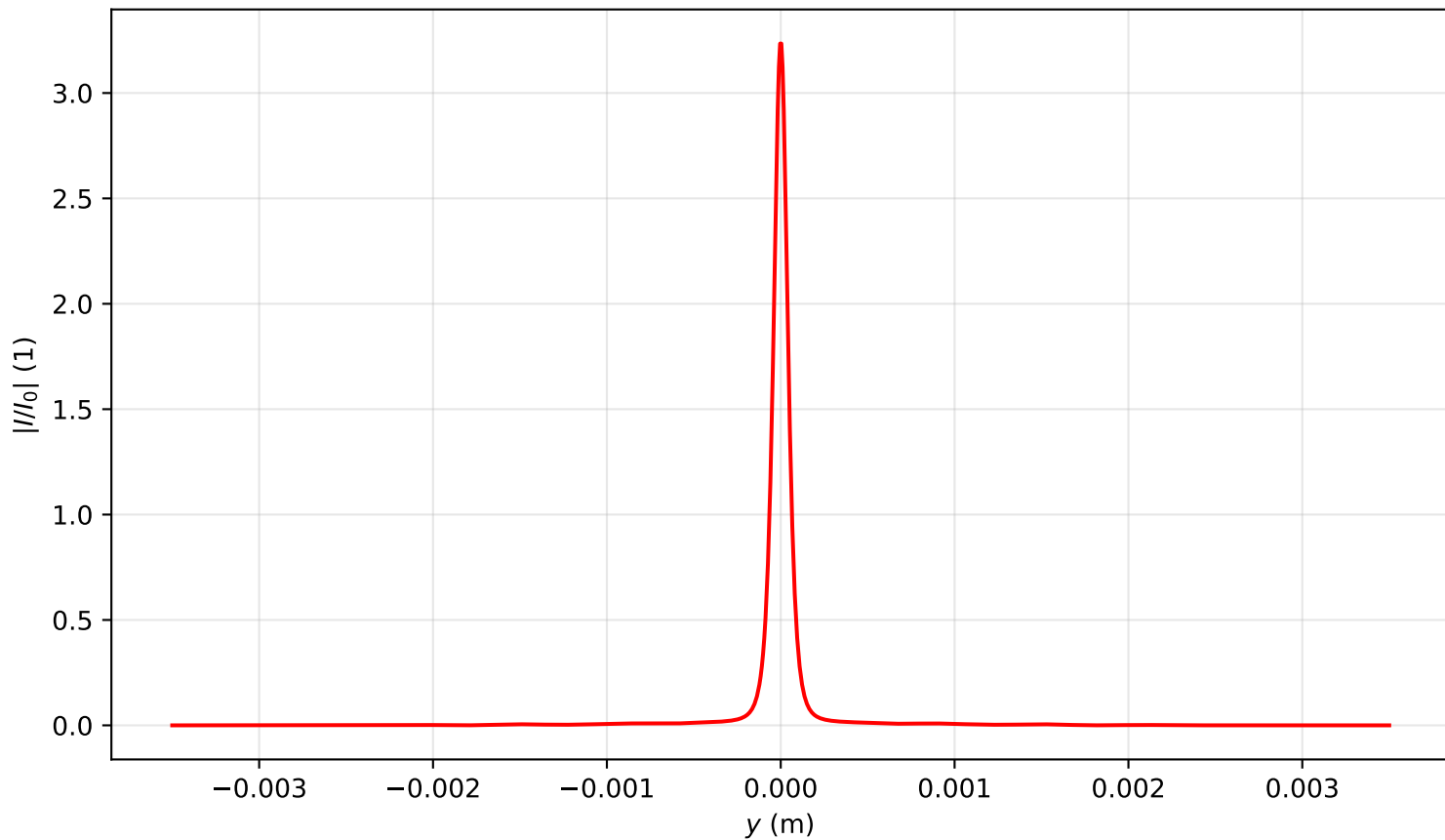
Intensity profile I(x=0, y, z=3.821)/I_0 , P_{in}=12.0P_{cr} , artificial time
