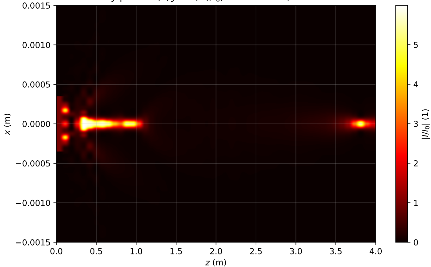
Intensity profile I(x, y = 0, z)/I_0 , P_{in}=12.0P_{cr} , artificial time
