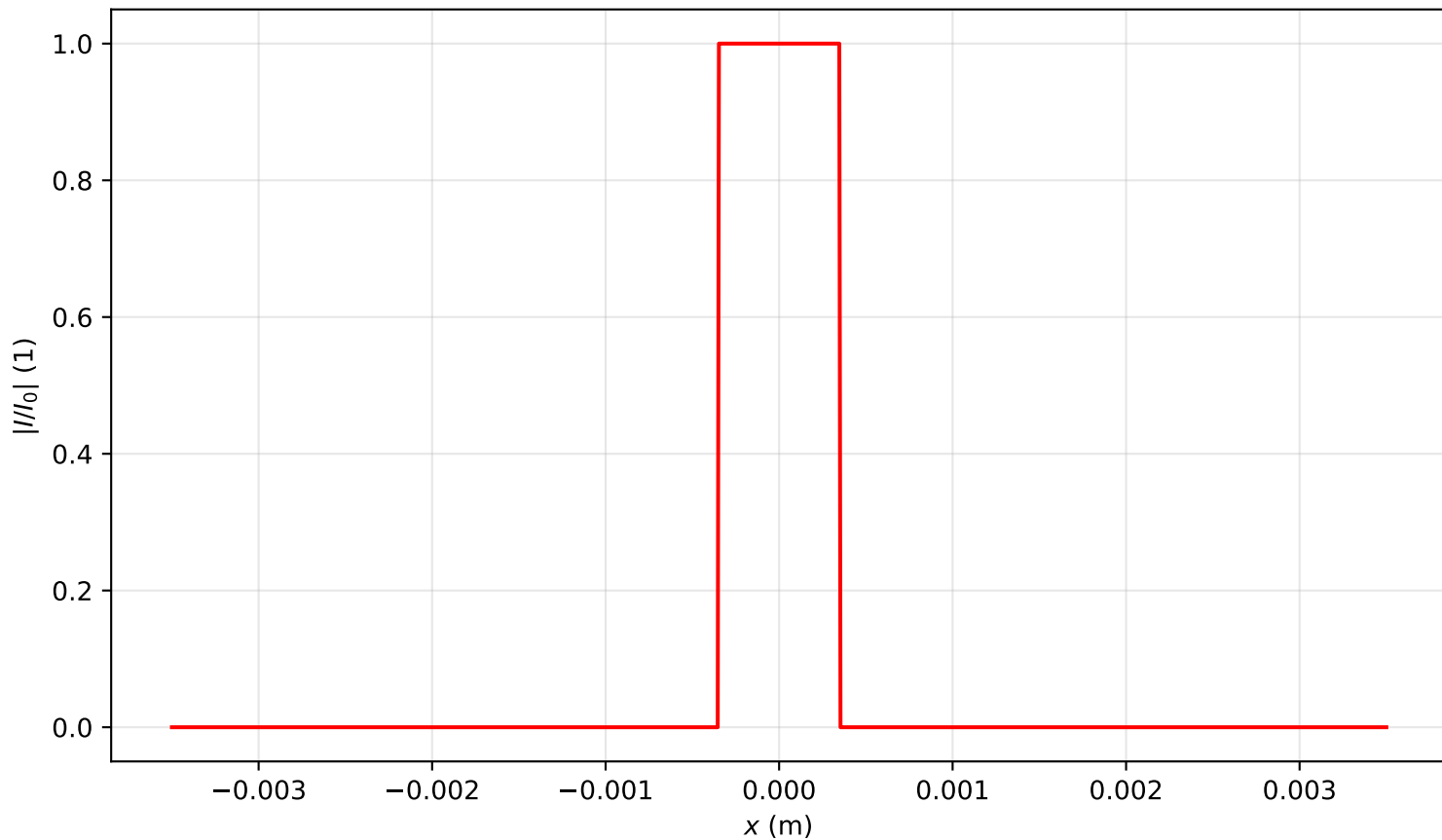
Intensity profile I(x, y = 0, z = 0.000)/I_0 , P_{in}=13.0P_{cr} , artificial time
