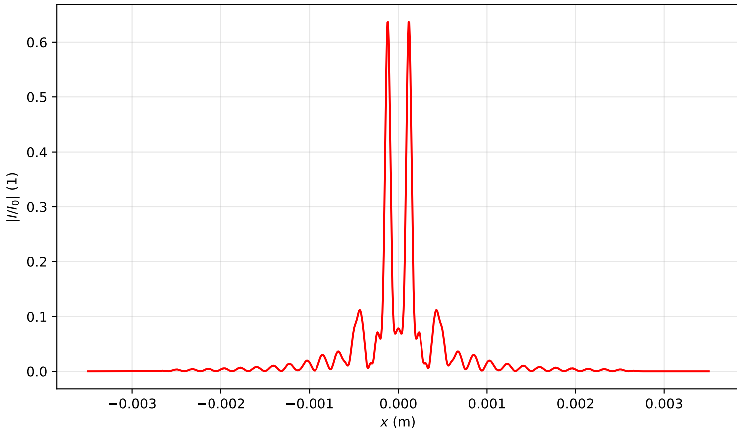
Intensity profile I(x, y = 0, z = 0.159)/I_0 , P_{in}=13.0P_{cr} , artificial time
