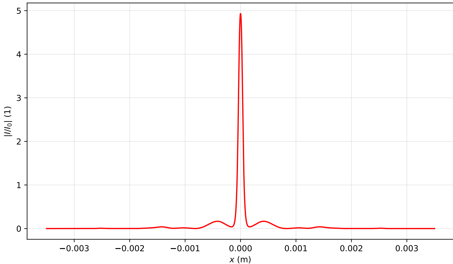
Intensity profile I(x, y = 0, z = 0.637)/I_0 , P_{in}=13.0P_{cr} , artificial time
