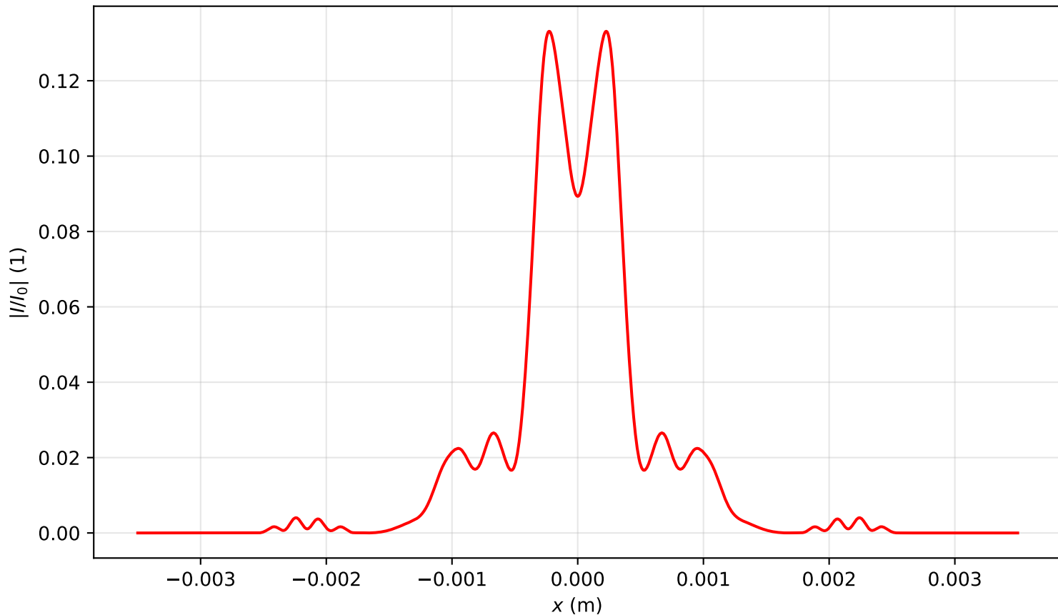
Intensity profile I(x, y = 0, z = 1.274)/I_0 , P_{in}=13.0P_{cr} , artificial time
