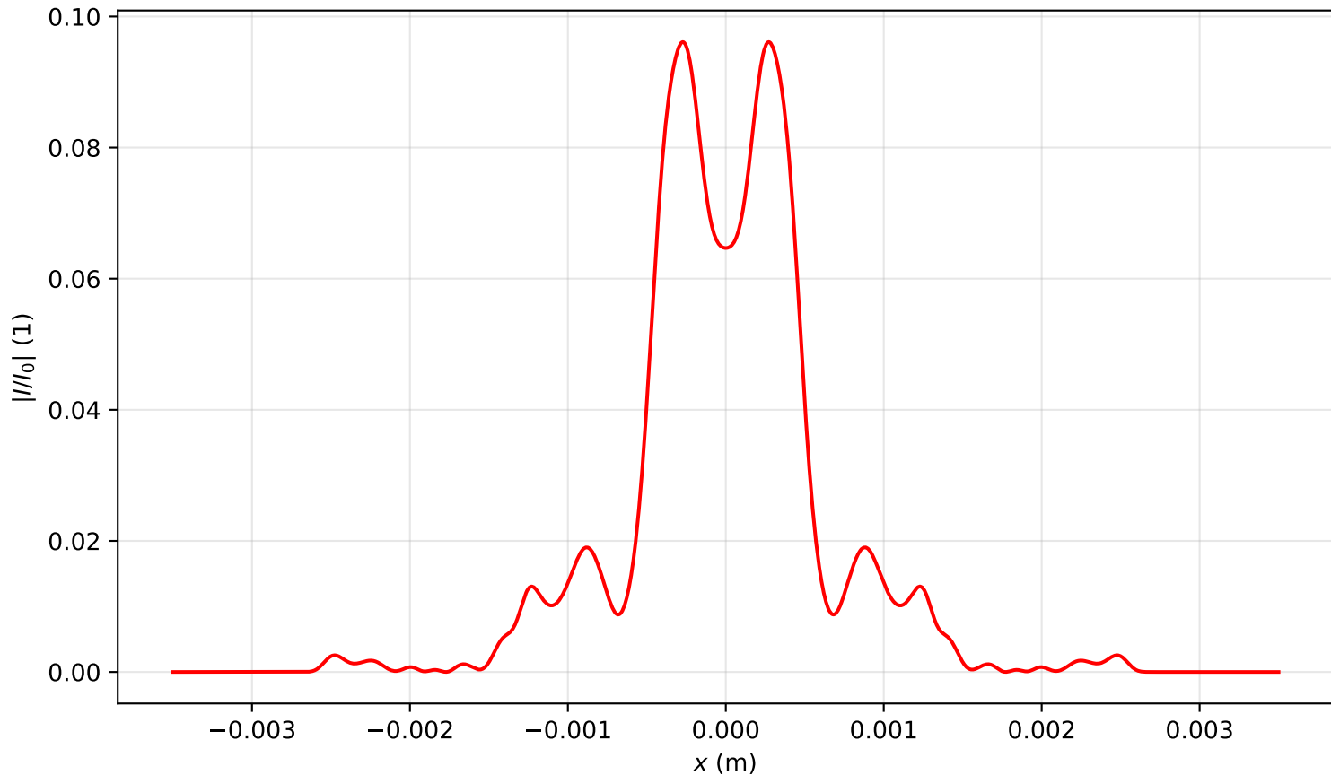
Intensity profile I(x, y = 0, z = 1.433)/I_0 , P_{in}=13.0P_{cr} , artificial time
