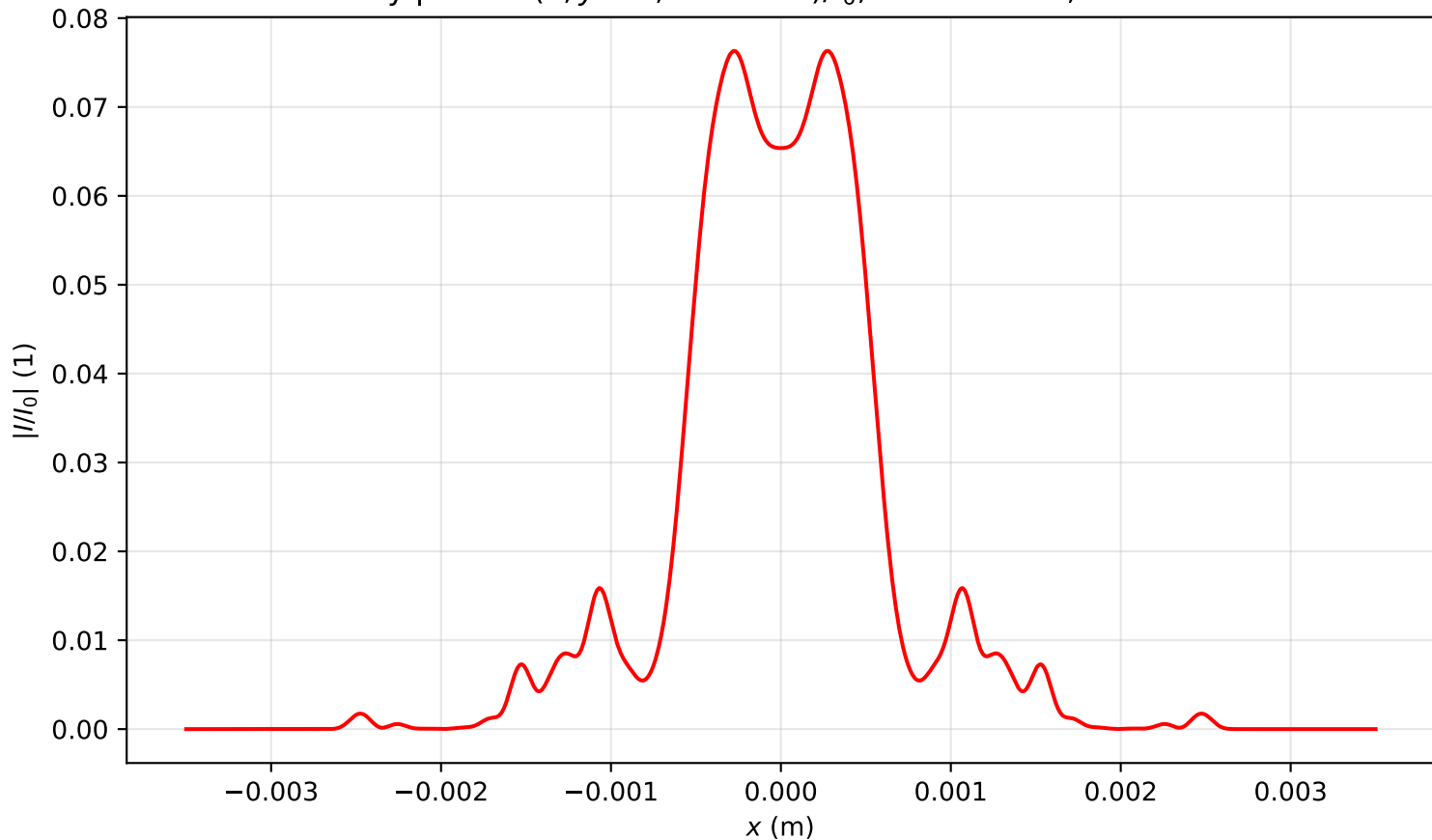
Intensity profile I(x, y = 0, z = 1.592)/I_0 , P_{in}=13.0P_{cr} , artificial time
