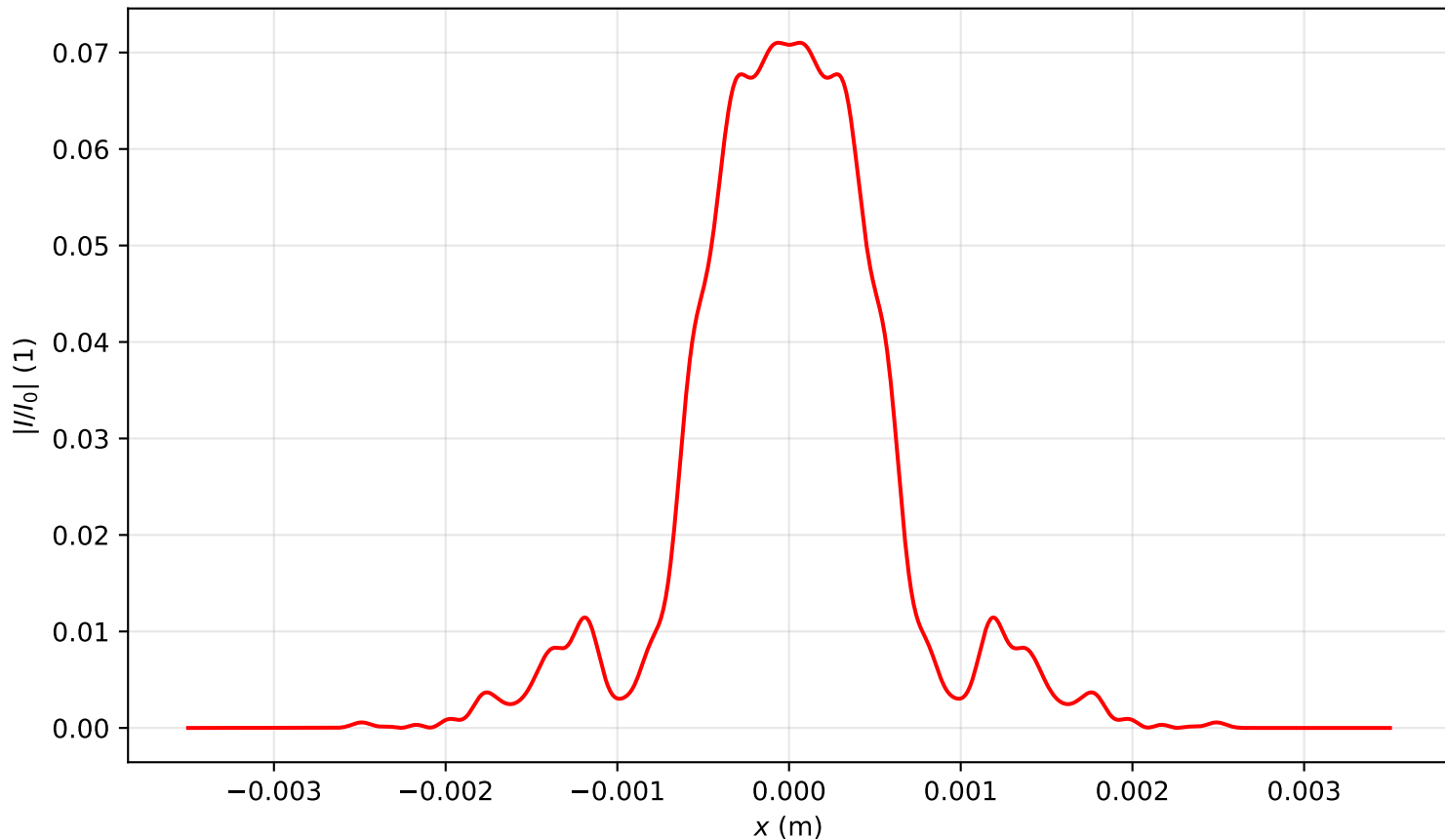
Intensity profile I(x, y = 0, z = 1.751)/I_0 , P_{in}=13.0\text{Pcr} , artificial time
