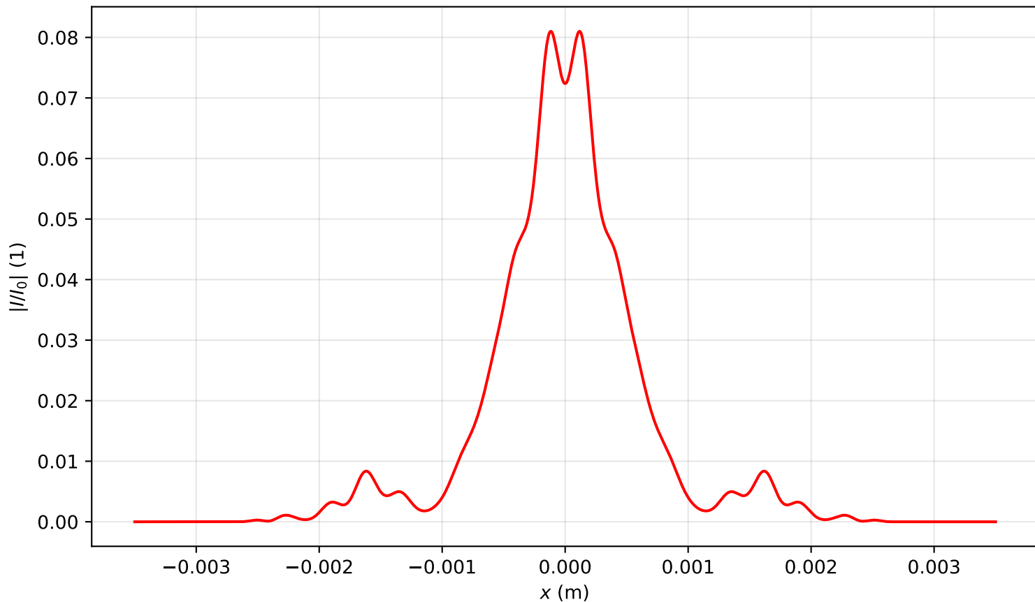
Intensity profile I(x, y = 0, z = 2.070)/I_0 , P_{in}=13.0P_{cr} , artificial time
