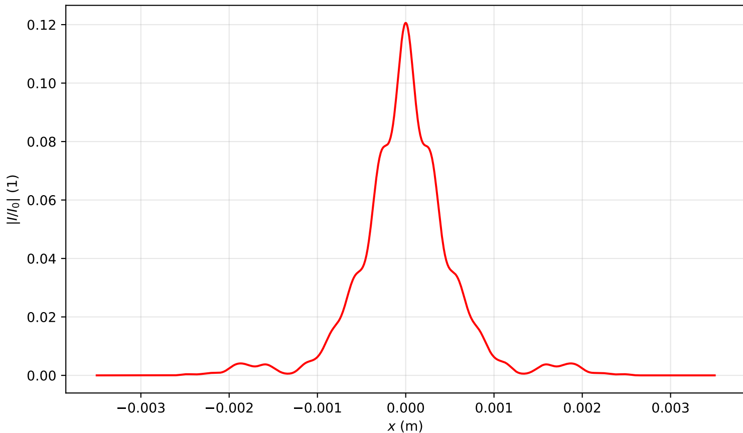
Intensity profile I(x, y = 0, z = 2.229)/I_0 , P_{in}=13.0P_{cr} , artificial time
