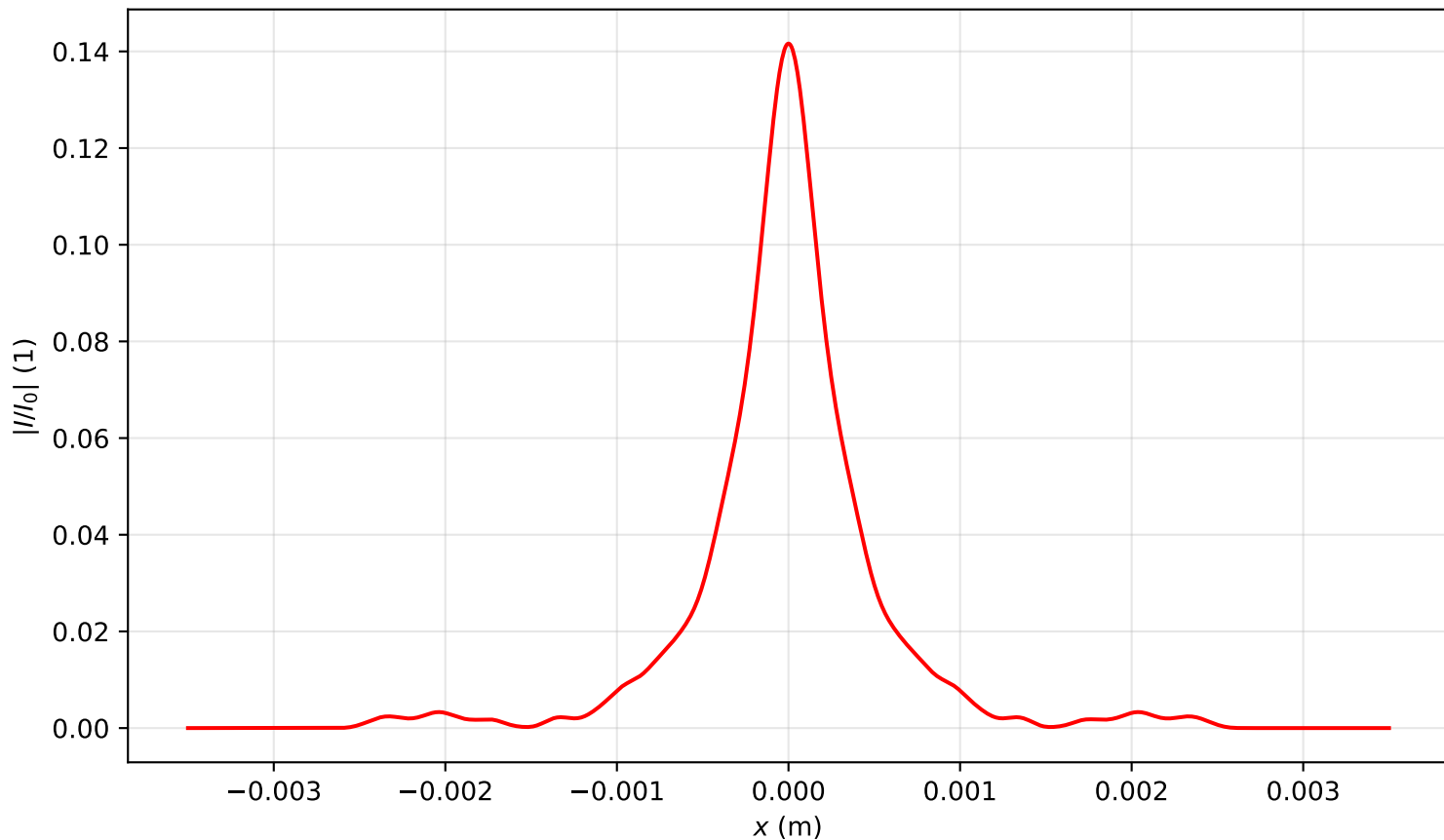
Intensity profile I(x, y = 0, z = 2.548)/I_0 , P_{in}=13.0P_{cr} , artificial time
