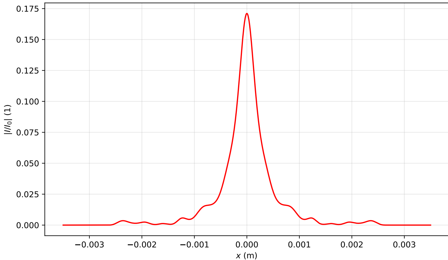
Intensity profile I(x, y = 0, z = 2.707)/I_0 , P_{in}=13.0P_{cr} , artificial time
