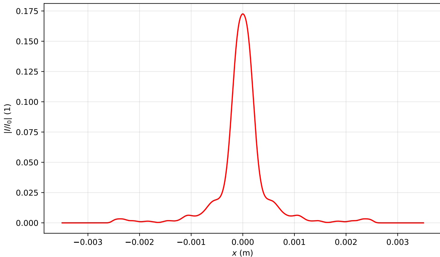
Intensity profile I(x, y = 0, z = 2.866)/I_0 , \text{Pin}=13.0\text{Pcr} , artificial time
