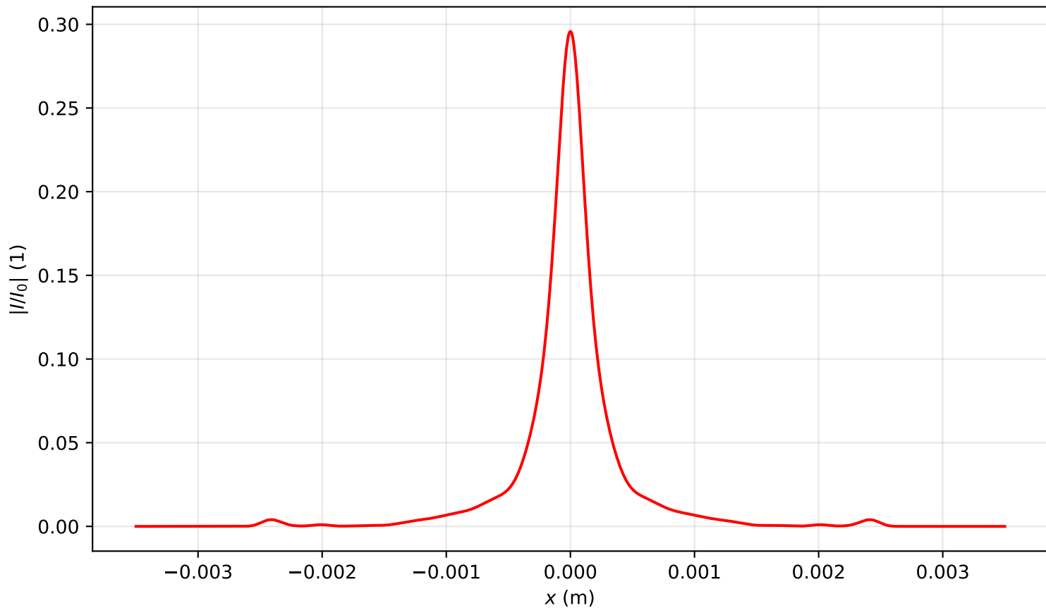
Intensity profile I(x, y = 0, z = 3.025)/I_0 , P_{in}=13.0P_{cr} , artificial time
