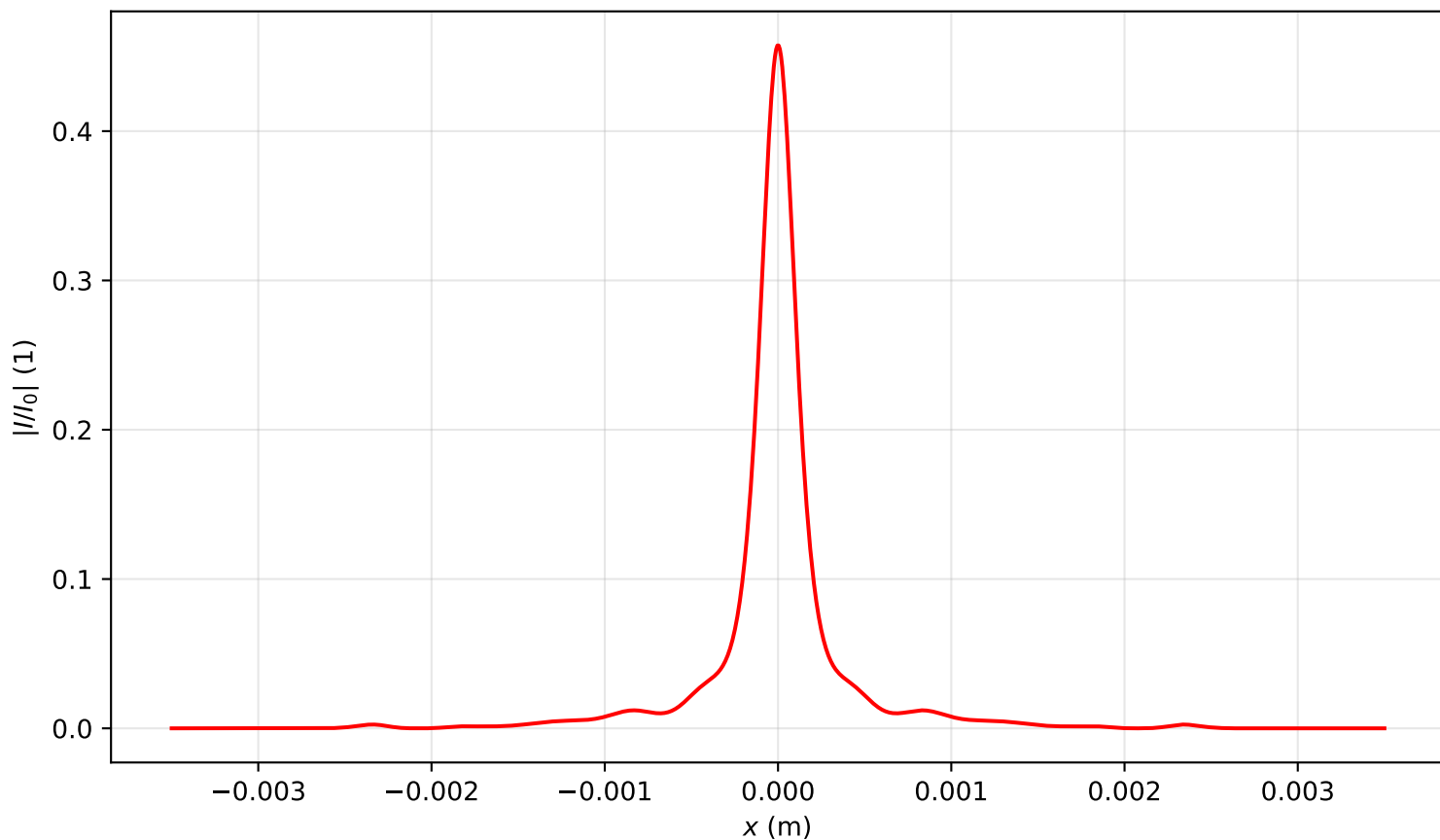
Intensity profile I(x, y = 0, z = 3.184)/I_0 , P_{in}=13.0P_{cr} , artificial time
